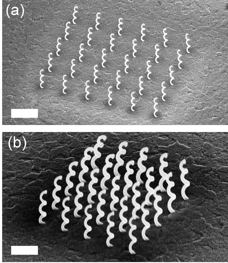
Figure 4.5: SEM micrographs of 5\times 5 helix arrays (a) and (b) fabricated with beam currents of 5 pA and 11 pA, respectively. The helix wires are thicker for the higher electron beam current. The acceleration energy for the structures shown in (a) and (b) is 3kV. The scale bars are 1\mu\text{m} .
